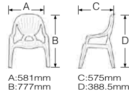
1188 Resin Arm Chair Size: 581L x 575W x 777H(mm) 12 pcs / 6.99 cuft / 0.198cbm
