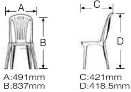
1184 Resin Chair Size: 491 x 421W x 837H(mm) 12pcs / 6.76 cuft / 0.192 cbm
