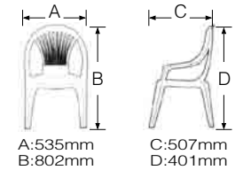
1189 Resin Arm Chair Size: 535L x 507W x 802H(mm) 12 pcs / 5.45 cuft / 0.155cbm
