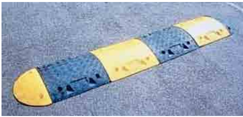
Expansion Bolts 10mm × 4nos Easy to install.Bolt down for permanent fixing.Checker plate pattern gives extra grip,integral reflectors.Suitable for light vehicles and HGV's.
