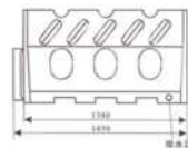
CODE:RB148A SIZE:1500MML*1000MMH CODE:RB148B SIZE:2000MML*1000MMH Easy storage Secure stacking for efficient transportation Link securely,even when on uneven ground Supplied with reflective strip Total Weight:15Kgs
